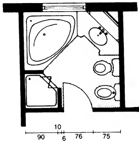
④ Small bathroom with corner bath
